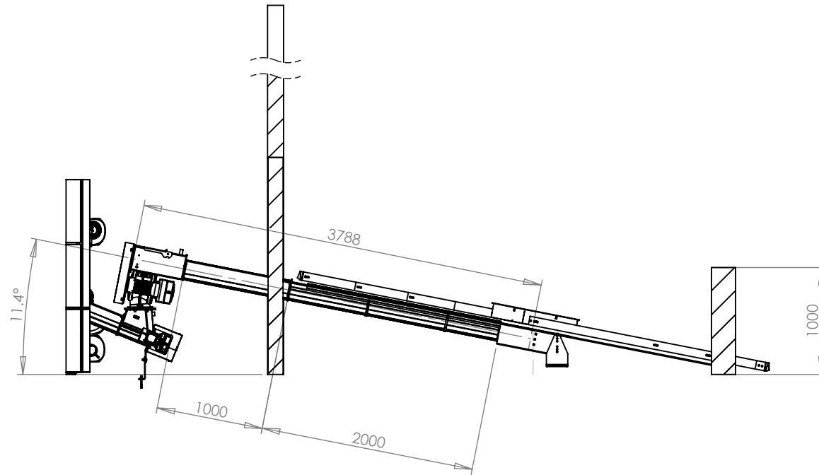
SECTION C-C Shows the length and installation angle of the feed system
